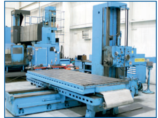
GIDDINGS & LEWIS MODEL 70-D5-T 5" TABLE TYPE HORIZONTAL BORING MILL
