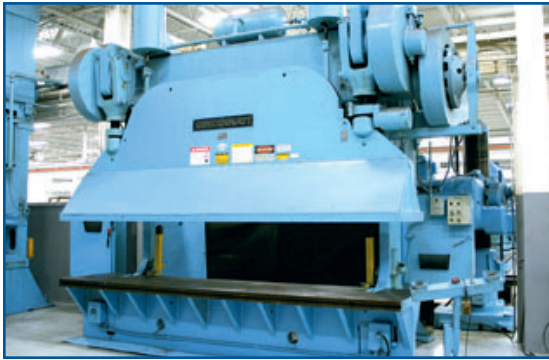
CINCINNATI 13 SERIES X 10' 400-TON X 14' MECHANICAL PRESS BRAKE
